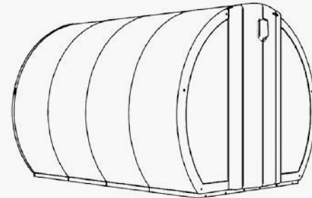
8 Person Outdoor Pod L3270mm x W2500mm x H2150mm Structure = 514kg Table = 64kg Lighting & Electrics = 2kg
