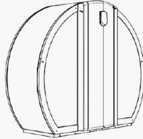
2 Person Outdoor Pod L1058mm x W2500mm x H2150mm Structure = 219kg Table = 16kg Lighting & Electrics = 2kg
