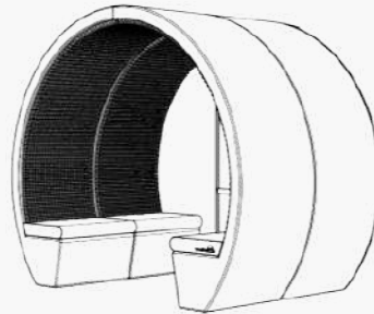
4 Person Meeting Pod L1570mm x W2500mm x H2100mm Structure = 220kg Table = 32kg LED lighting = 2kg
