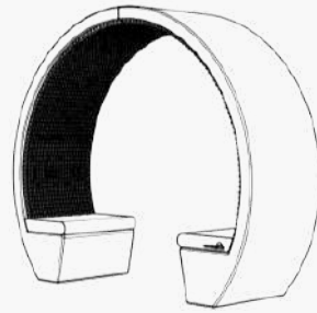
2 Person Meeting Pod L750mm x W2500mm x H2100mm Structure = 60kg Table = 16kg LED lighting = 2kg
