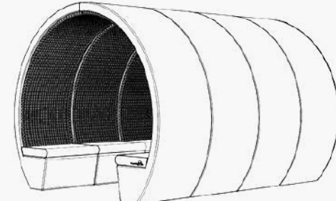
8 Person Meeting Pod L3000mm x W2500mm x H2100mm Structure = 240kg Table = 58kg LED lighting = 2kg
